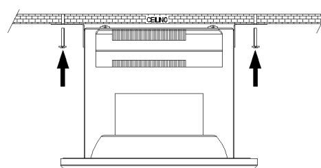
POP Mount Light - Installed Condition
