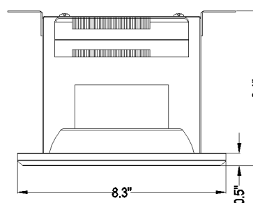
POP Mount Light - Installed Condition
