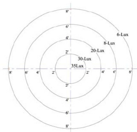
Test Height: 8-Foot Iso-Lux Graph
