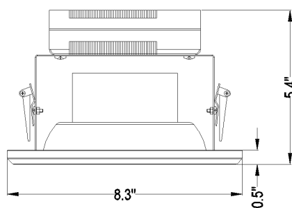
Surface Mount Light - Installed Condition
