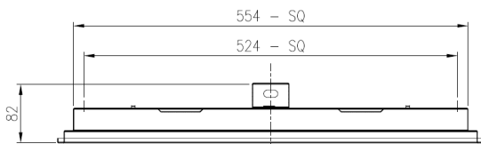
Surface Mount Light - Installed Condition
