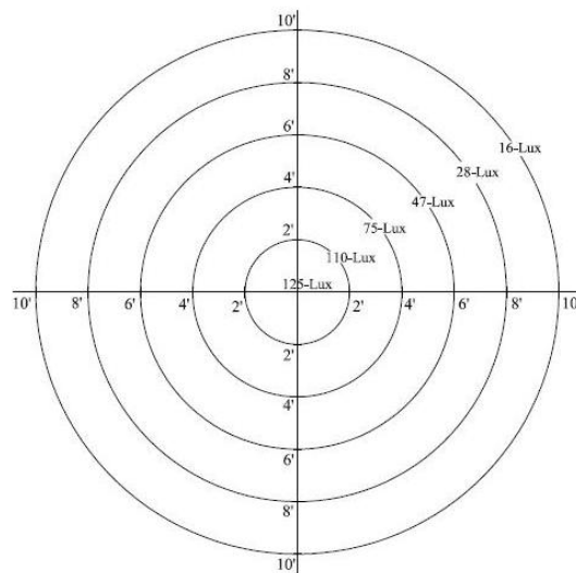
Test Height: 8-Feet Iso-Lux Graph
