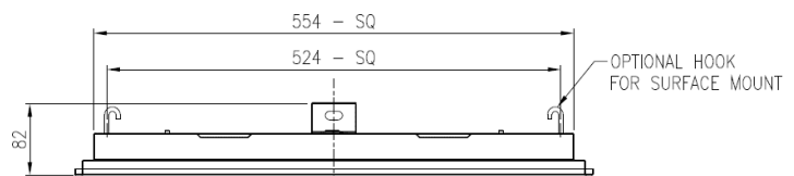
POP Mount Light - Installed Condition
