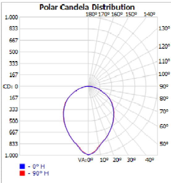
Figure 1 : Luminous Intensity Diagram
