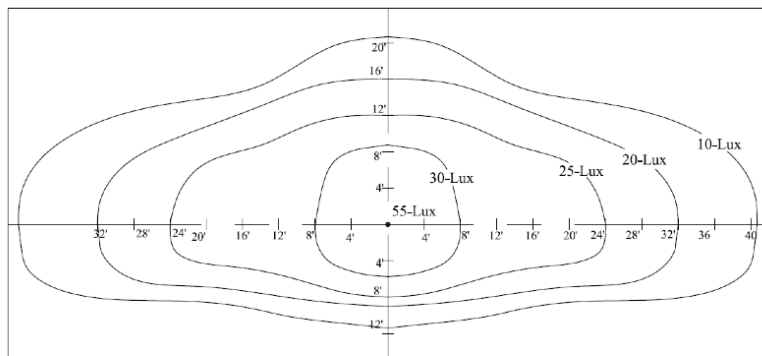
Iso-Lux Diagram @ 24 Feet Mounting Height
