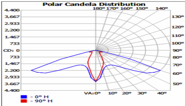
Figure 1 : Luminous Intensity Diagram
