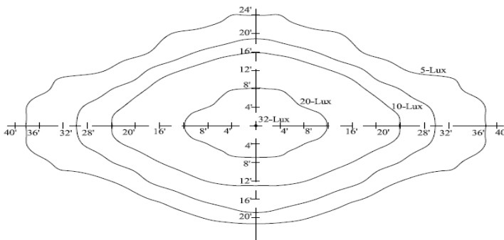
Iso-Lux Diagram @ 24 Feet MH
