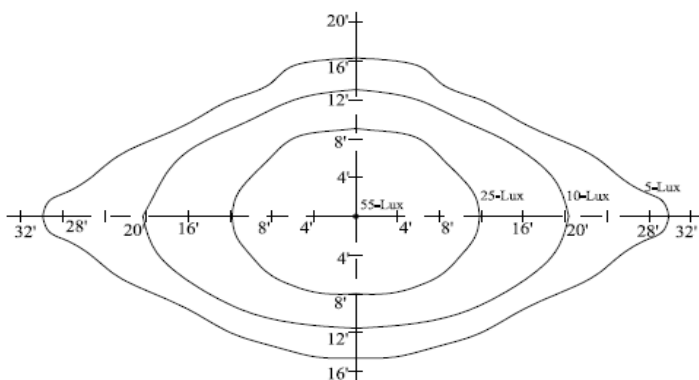
Iso-Lux Diagram @ 18 Feet MH
